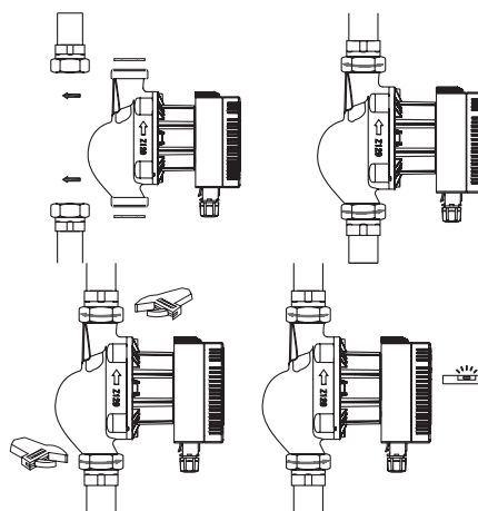
Fig. 35 Pump installation
