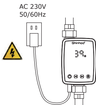
Fig.6 Wiring Diagram
