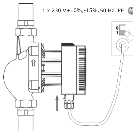
Fig. 36 Electrical connection
