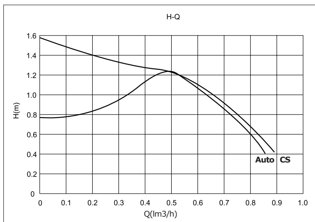
Fig.4 Performance curve
