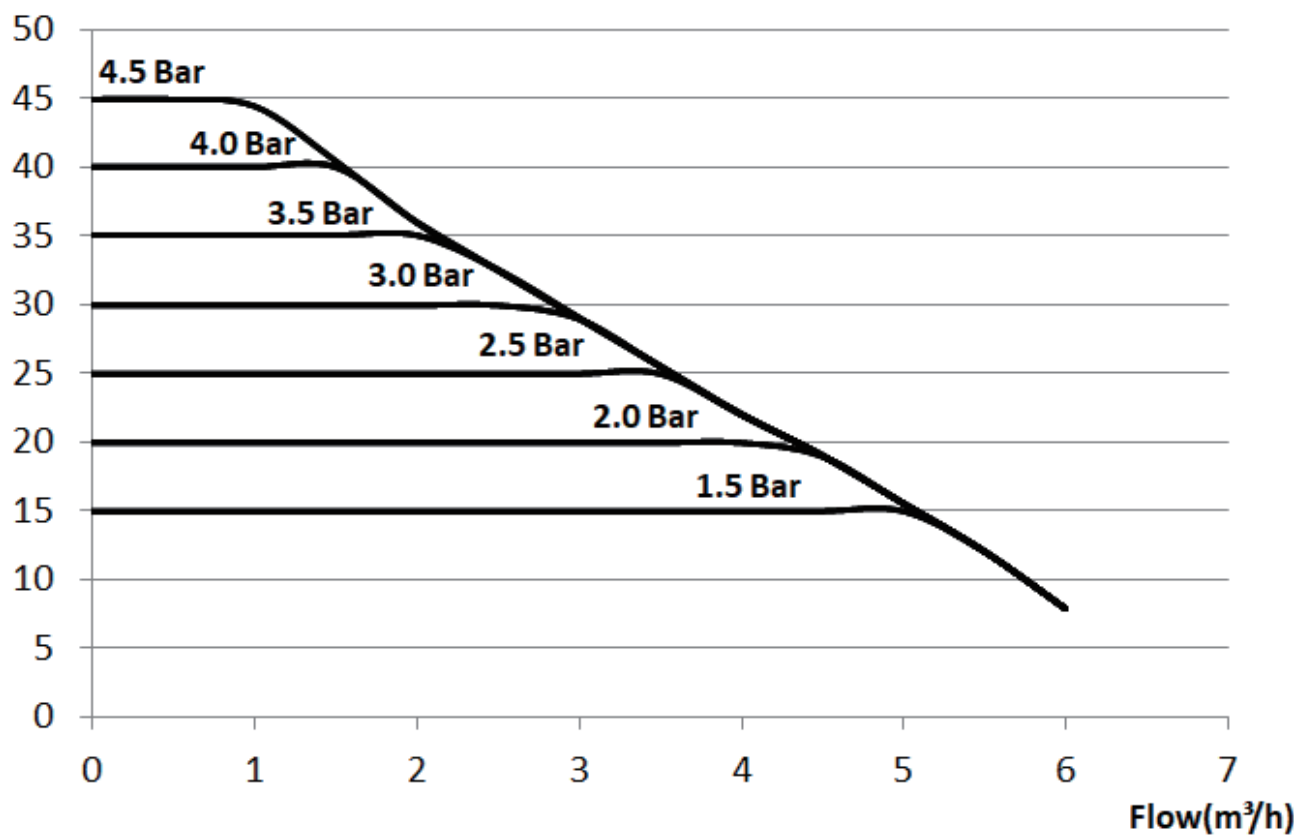
Fig.6 Performance curves
